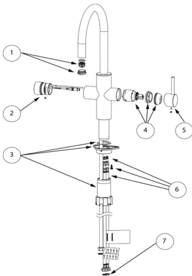
Maris MFT electronic J-spout SS 119.0698.122
